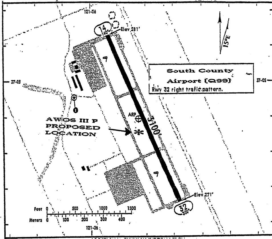
Automatic Weather Observation System (AWOS) III P
