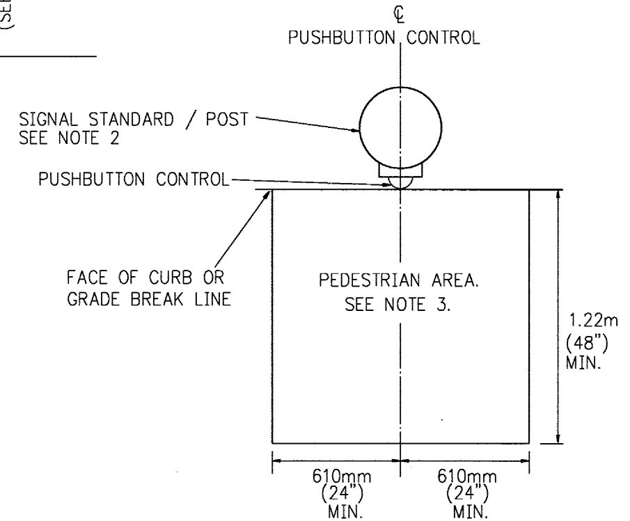
B TOP VIEW - PUSHBUTTON CONTROL MOUNTING HORIZONTAL CLEARANCE
