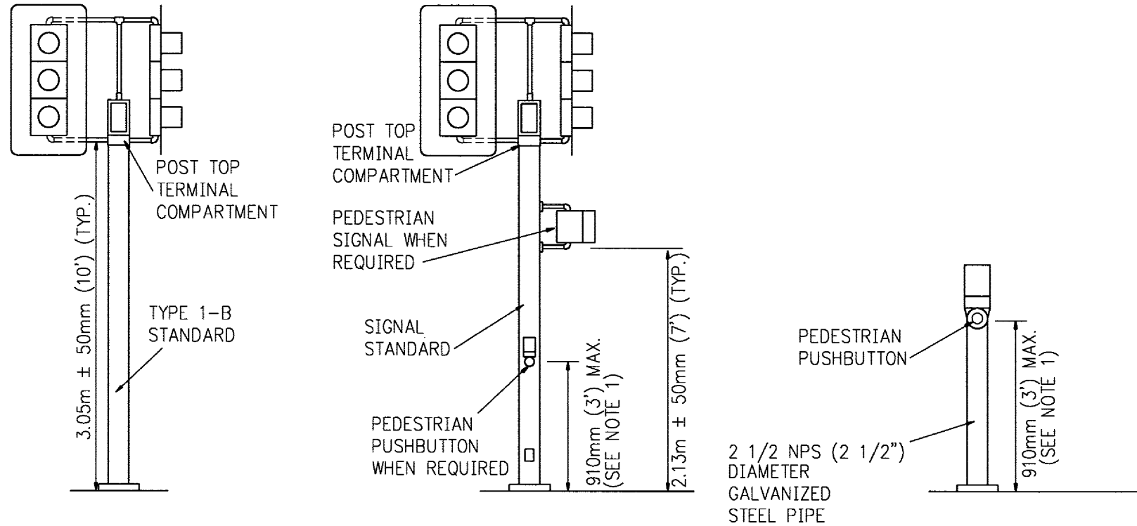
A SIGNAL MOUNTING VERTICAL CLEARANCE
